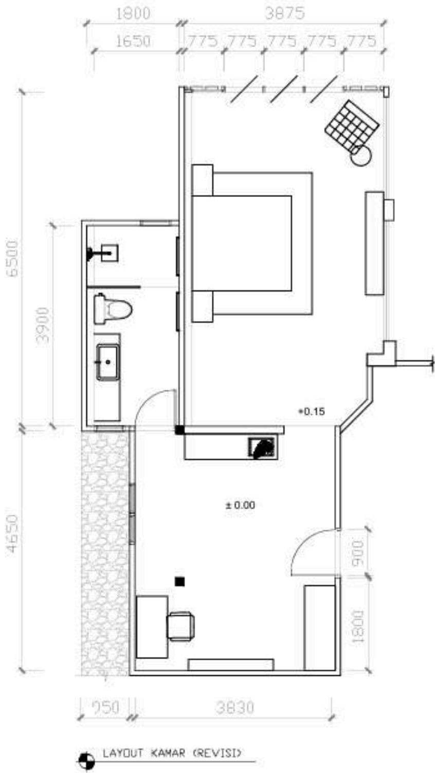
Technical drawings – Plan layout and Section
