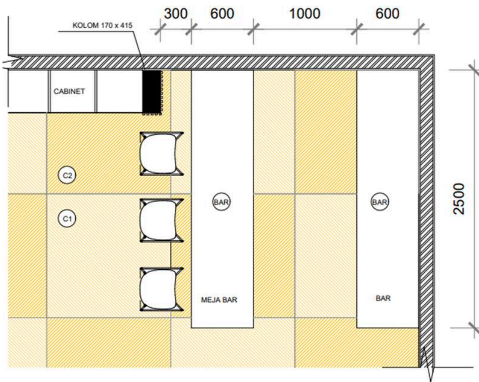
BAR AREA PLAN SCALE 1 : 25 BAR TOP (BAR) 600 X 2500 MM (MARBLE TOP) FLOOR CUT SIZES C1 1200 X 1200 MM C2 1200 X 1200 MM
